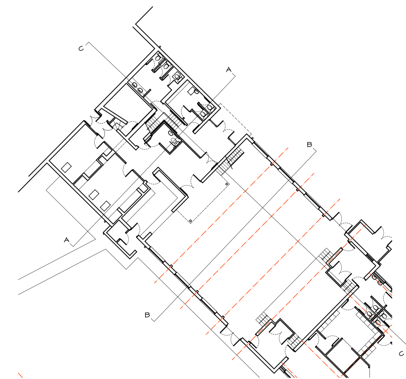
04 Mackworth Community Centre, Mackworth Key Plan 1:200
